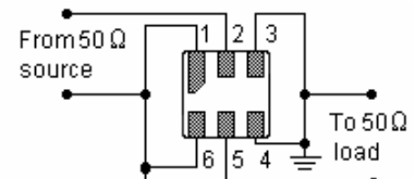
Test Circuit
