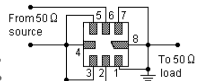
Test Circuit
