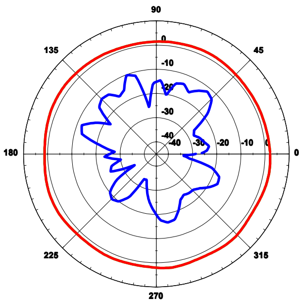
H - Plane
