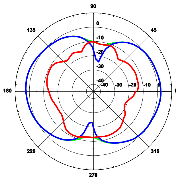
E - Plane
